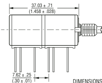
Dual Section Model 83 PC Pins
