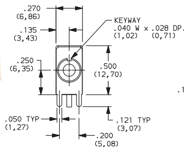
8121SD9AVGE SPDT
