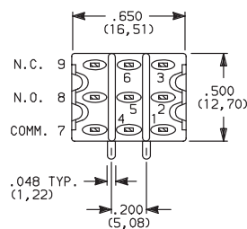
PC MOUNTING
