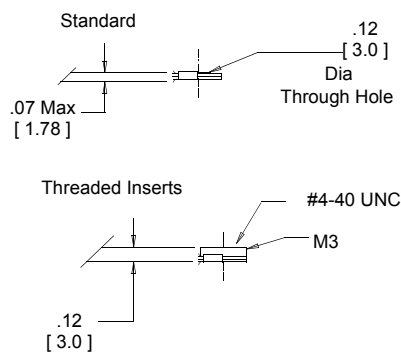
Mounting Styles
