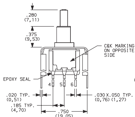
8261SH9_BE2 DPDT
