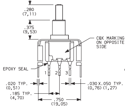
8161SH9_BE2 SPDT
