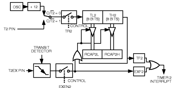
Figure 8. Timer in Auto-Reload Mode.
