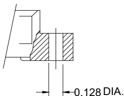
VARIATION 02 .128±.003 DIA. MOUNTING HOLE
