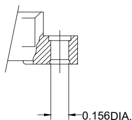
VARIATION 04 .156 +.002 -.000 DIA. MOUNTING HOLE
