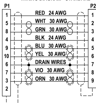
WIRING DIAGRAM - STANDARD
