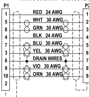
WIRING DIAGRAM - CROSSOVER
