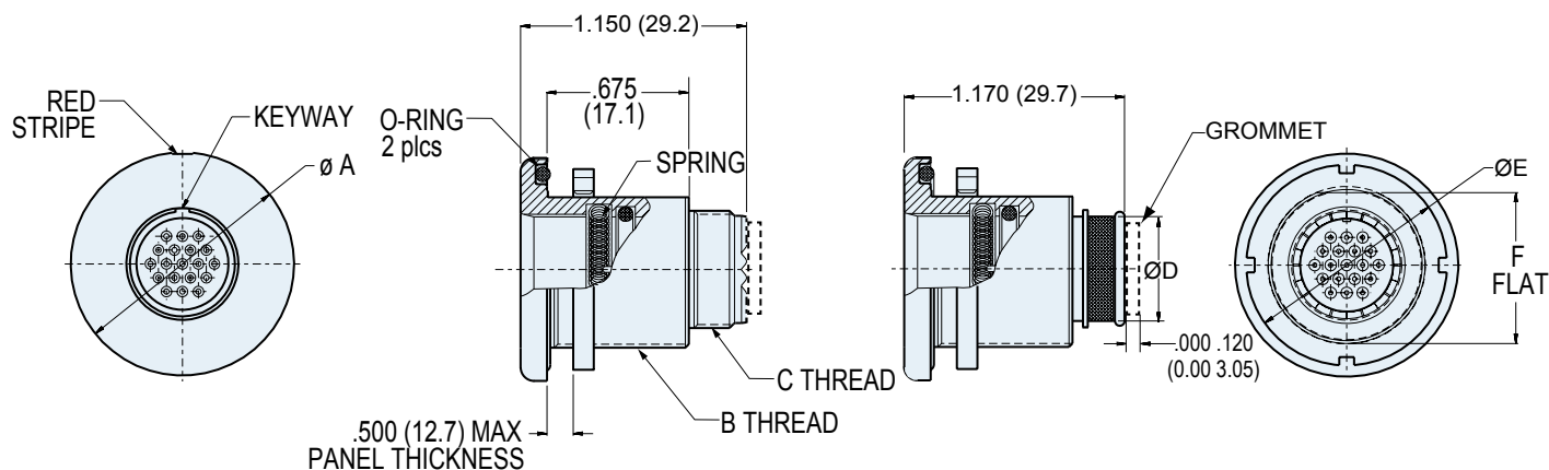
Accessory Thread 804-004-00
