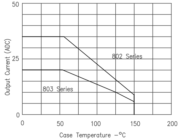
Figure 3 Current Derating
