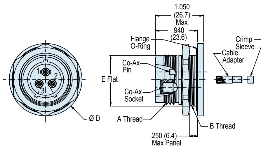
Rear Panel Jam Nut Mount Submersible Hermetic 802-040-07
