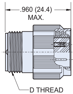
Accessory Thread 801-008
