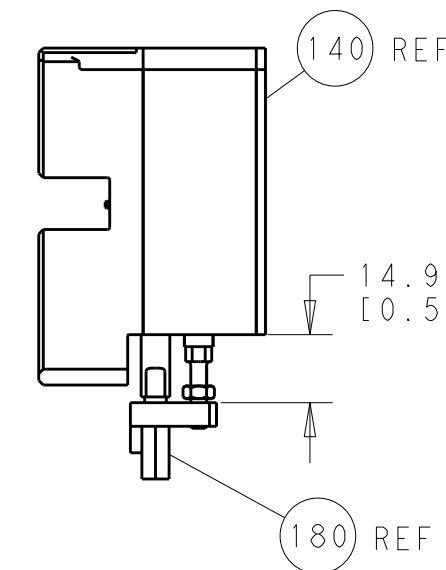
HOLDDOWN SET-UP
