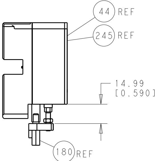
HOLDDOWN SET-UP
