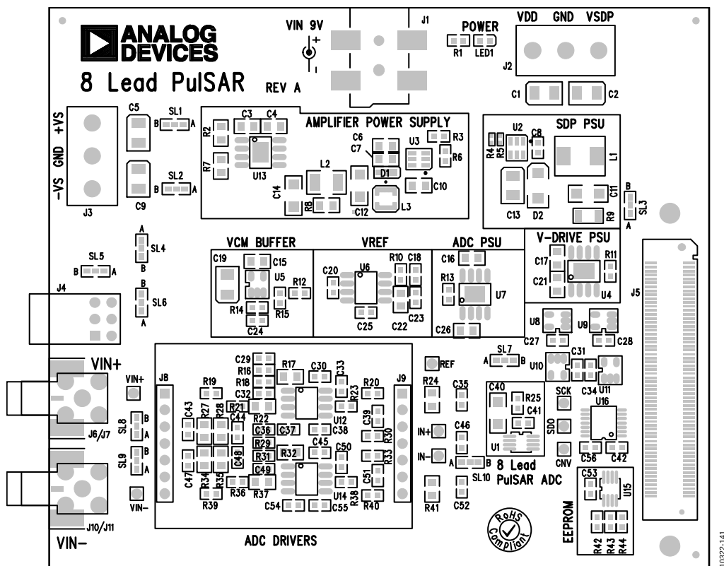
Figure 41. 8-Lead Evaluation Board Silkscreen, Top Layer
