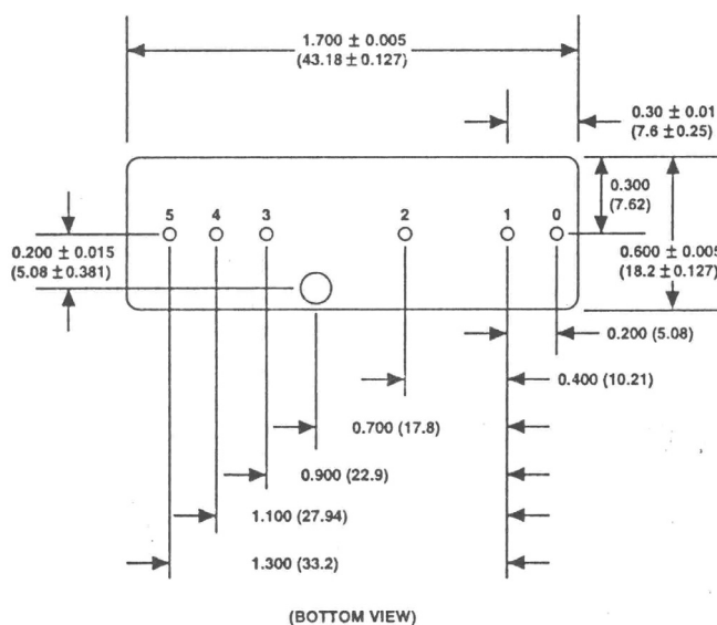
Figure 4 . Model 7B Series Module, with pin-out assignments.
