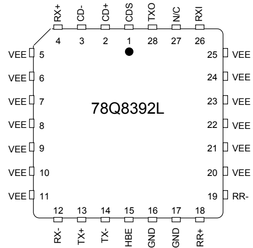
28-Pin PLCC
