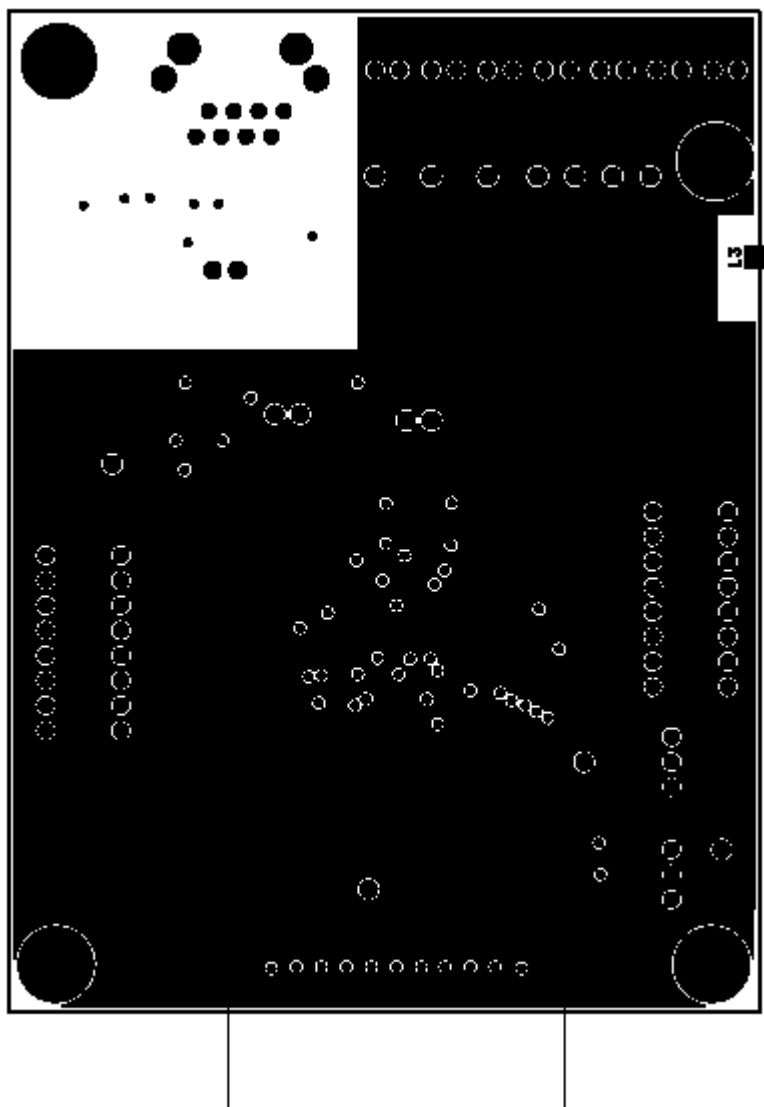
Ground Layer
