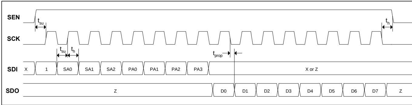
Read Operation
