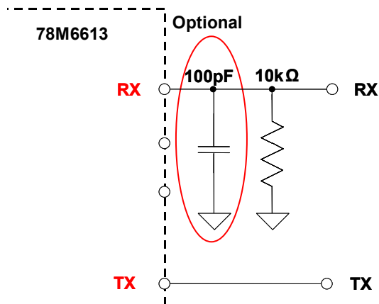
Figure 10: Connections for the RX Pin
