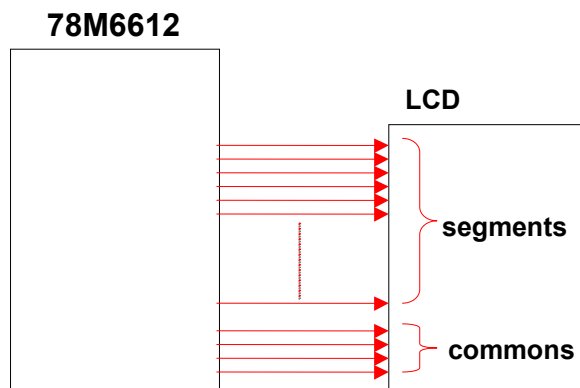
Figure 11: Connecting LCDs
