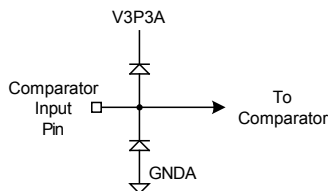
Comparator Input Equivalent Circuit
