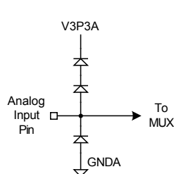
Analog Input Equivalent Circuit
