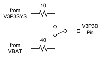
V3P3D Equivalent Circuit
