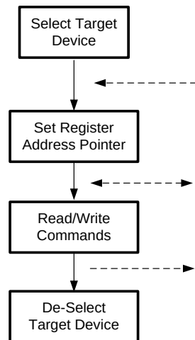
Figure 29. SSI Protocol
