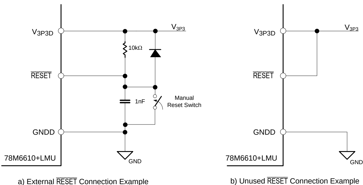
Figure 7. Reset Connections
