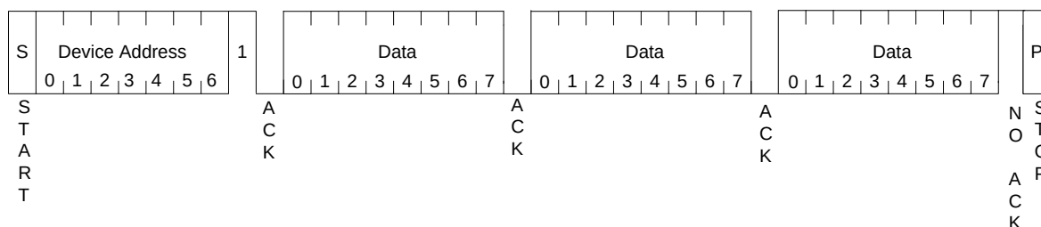
Figure 40. Read Operation
