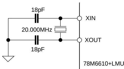
Figure 6. Crystal Connections
