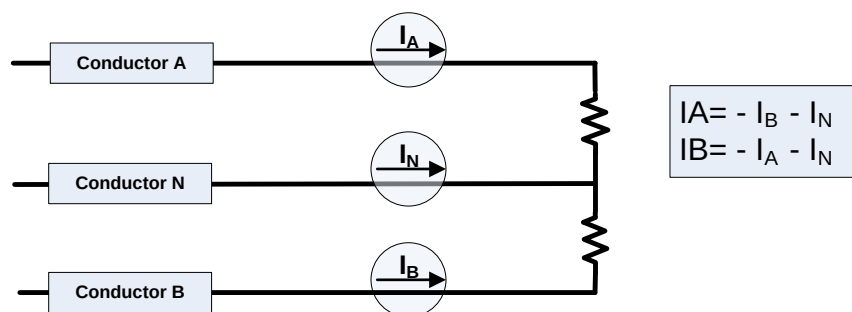
Figure 13. Current Input Configuration
