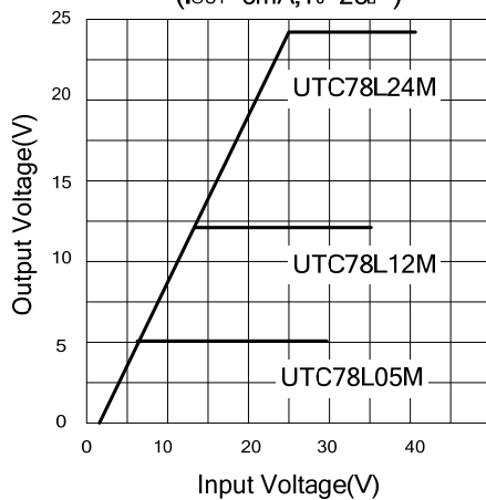
Fig.3 Output Characteristics ( I_{OUT}=0mA, T_J=25^\circ C )
