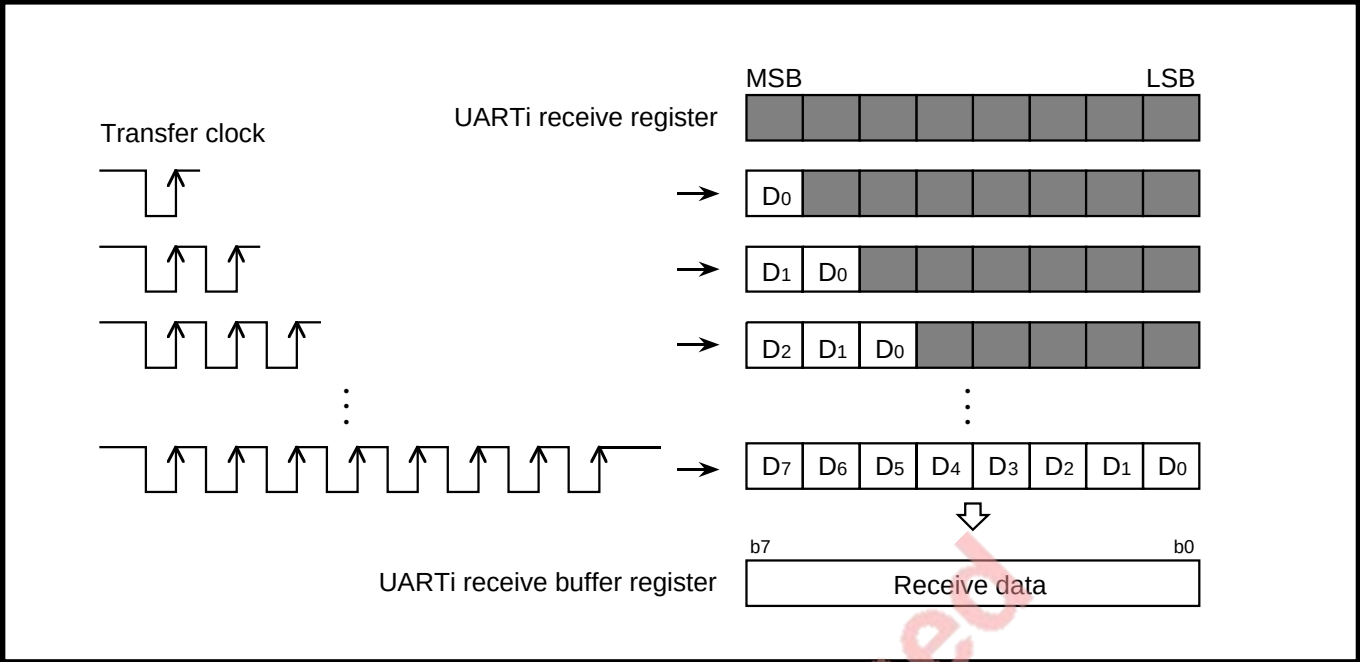
Fig. 7.3.10 Receive operation
