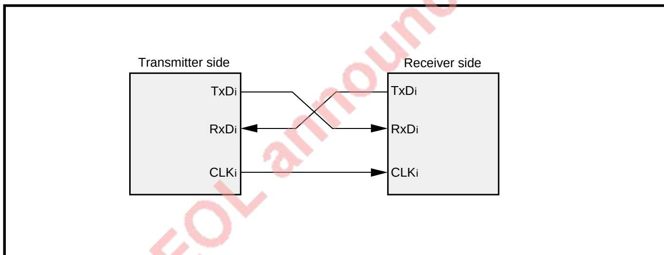
Fig. 7.3.9 Connection example
