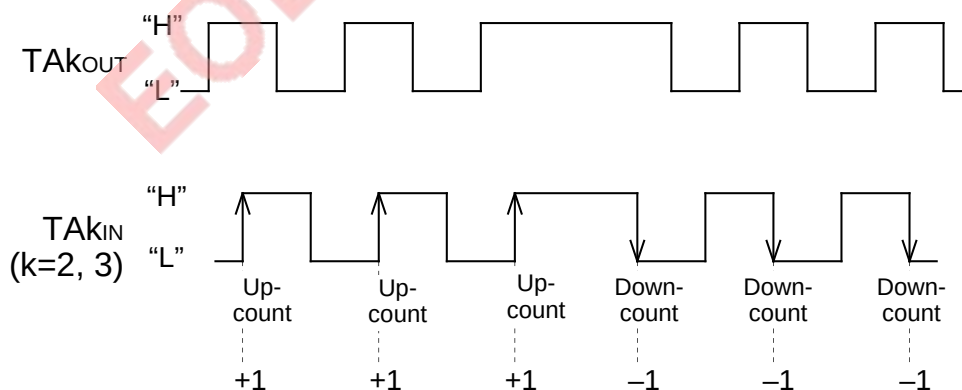
Fig. 5.4.7 Normal processing
