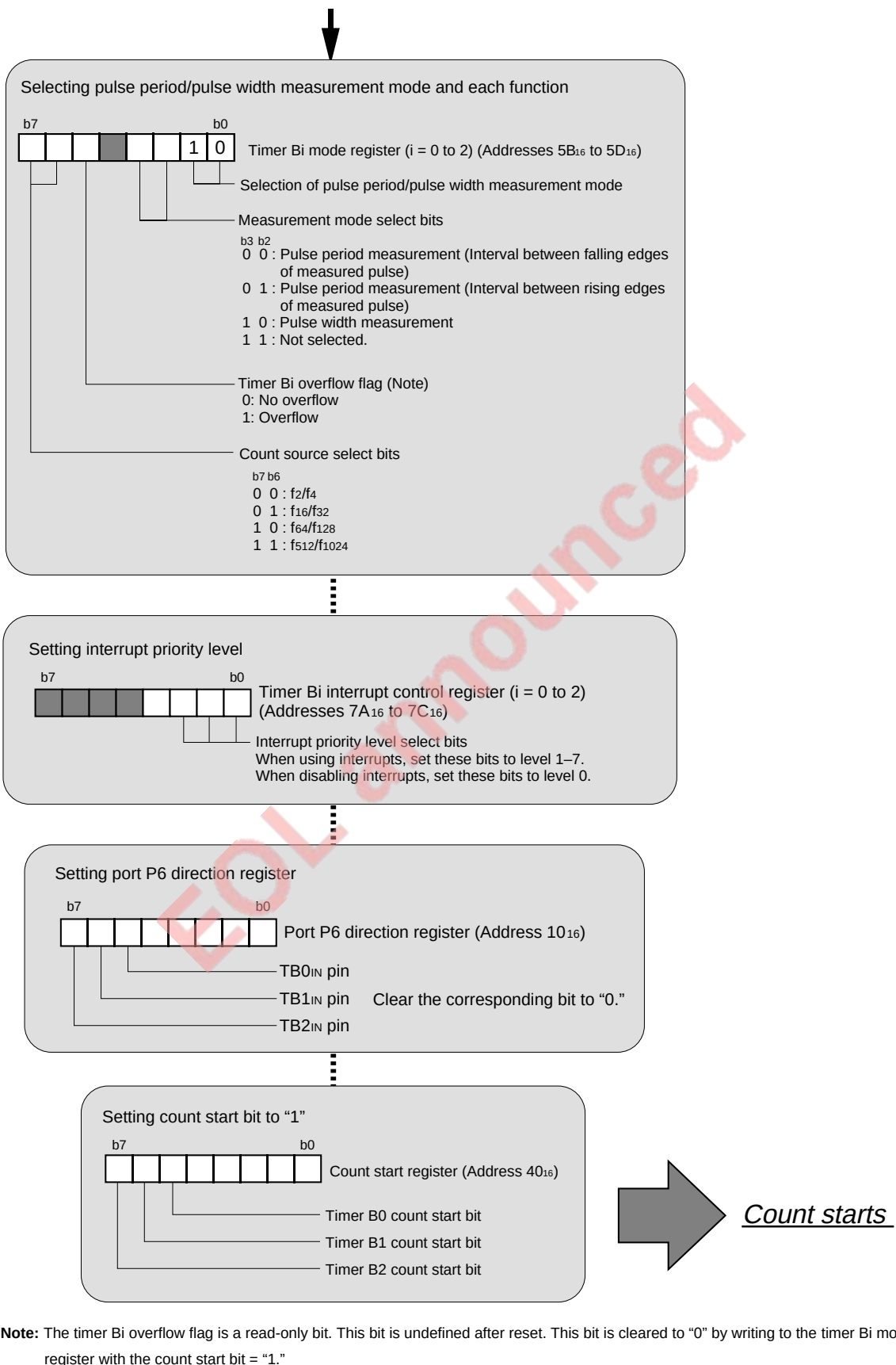
Fig. 6.5.2 Initial setting example for registers relevant to pulse period/pulse width measurement mode
