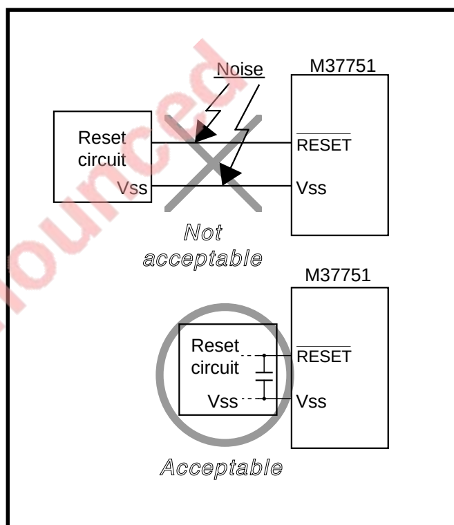
Fig. 5. Wiring for RESET pin
