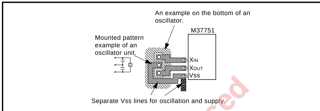
Fig. 14. Vss pattern underneath mounted oscillator
