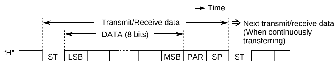
Fig. 7.4.2 Example of transfer data format
