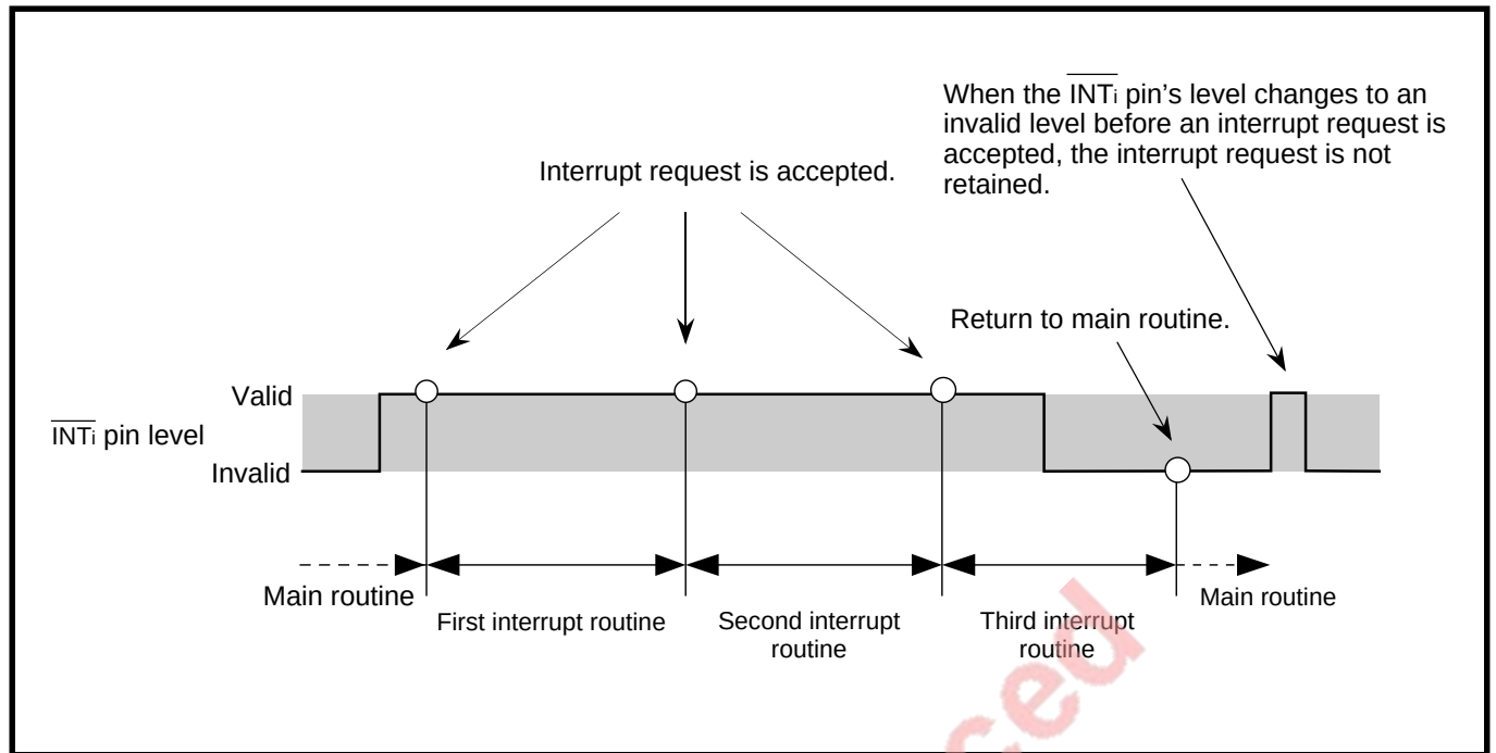
Fig. 4.10.4 Occurrence of \overline{\text{INT}}_i interrupt request in level sense mode
