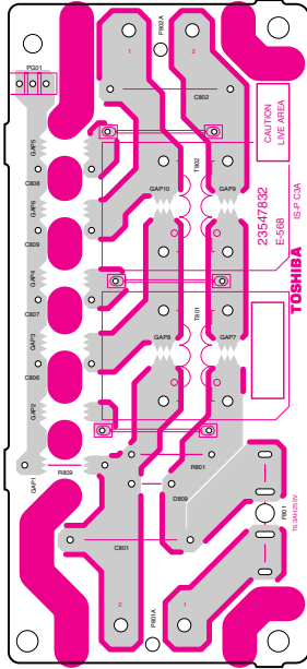
AC-IN BOARD PD2171C2 (U802) BOTTOM (FOIL) SIDE
