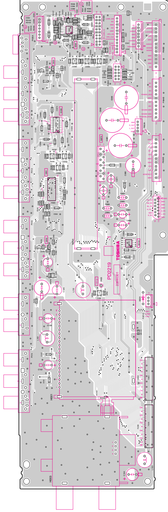
TN/AV-AOUT BOARD PD2219A1 (U104A) TOP (COMPONENT) SIDE
