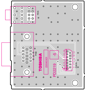
PC-IN BOARD PD2219A5 (U104E) TOP (COMPONENT) SIDE
