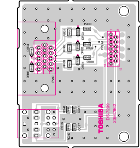
PC-IN BOARD PD2219A5 (U104E) BOTTOM (FOIL) SIDE
