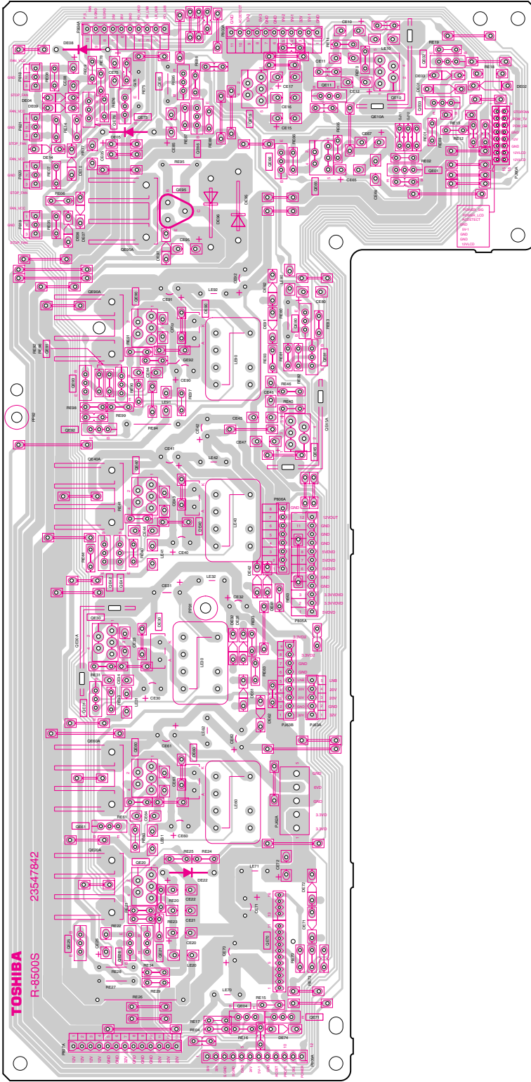
LOWB BOARD PD2189B1 (U803) BOTTOM (FOIL) SIDE
