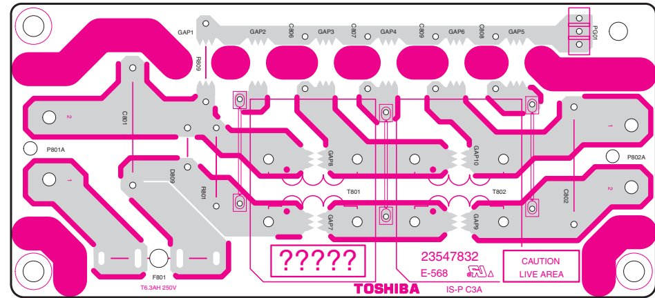
AC IN BOARD PD2171D2 (U002B)
