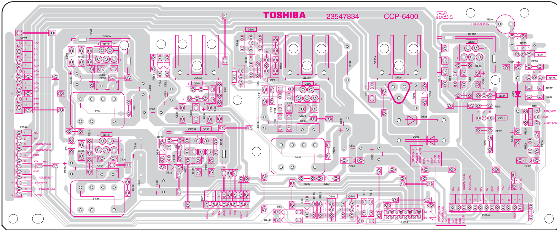
LOW B BOARD PD2173C1 (U004)
