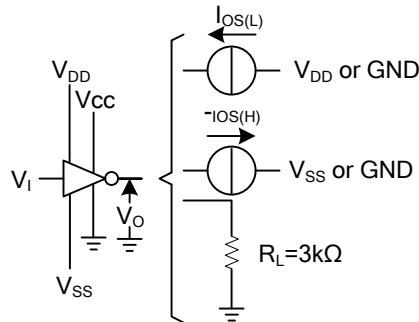
Fig. 1 Driver Test Circuit for V_{OH} , V_{OL} , I_{OH(H)} , I_{OL(L)}
