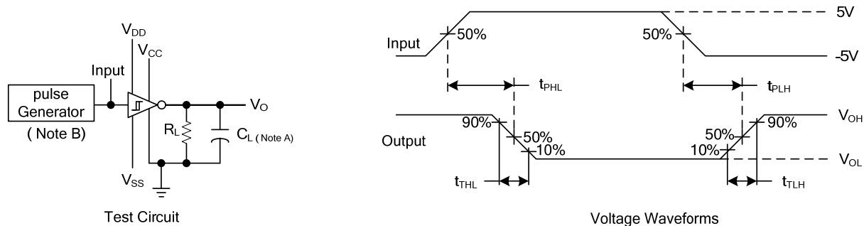
Fig. 6 Receive Propagation and Transition Times
