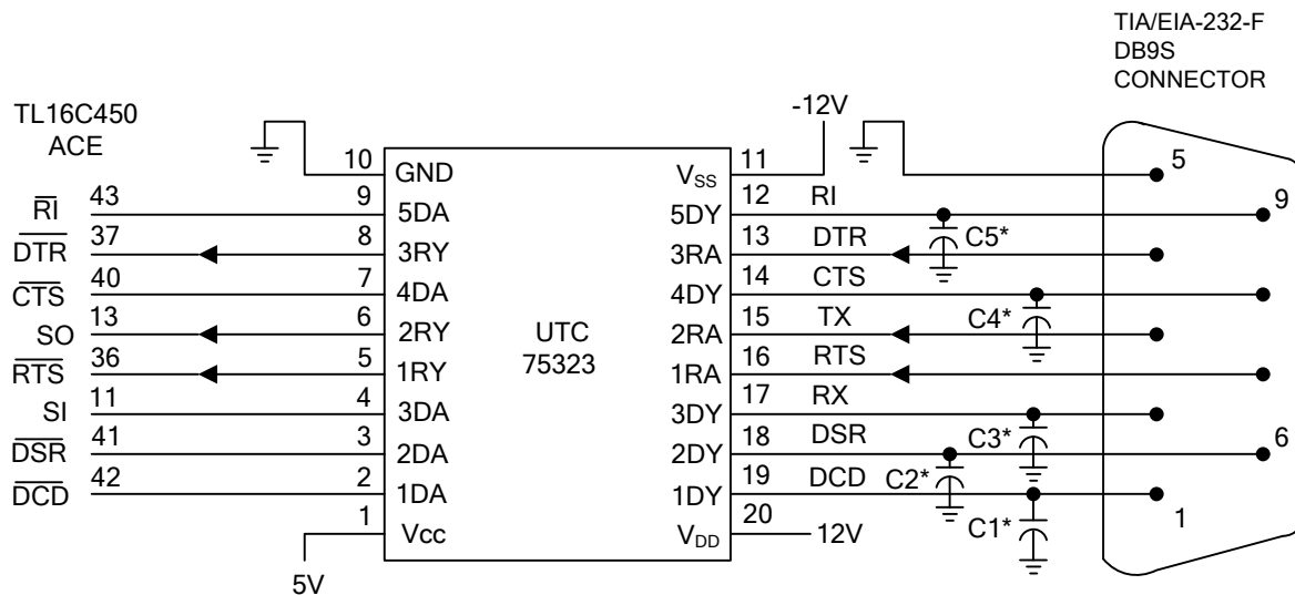
Fig. 8 Typical Connection
