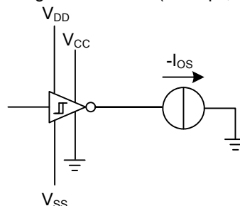
Fig. 4 Receiver Test Circuit for I_{OS}
