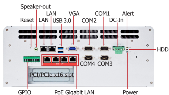
EC320/321-CR4866 Rear View
