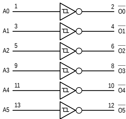
Figure 2. Logic Diagram
