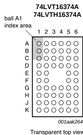
Fig 5. Pin configuration for SOT702-1 (VFPGA56)
