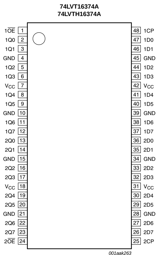
Fig 4. Pin configuration for SOT370-1 (SSOP48) and SOT362-1 (TSSOP48)
