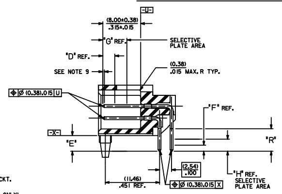
SECTION Z-Z
