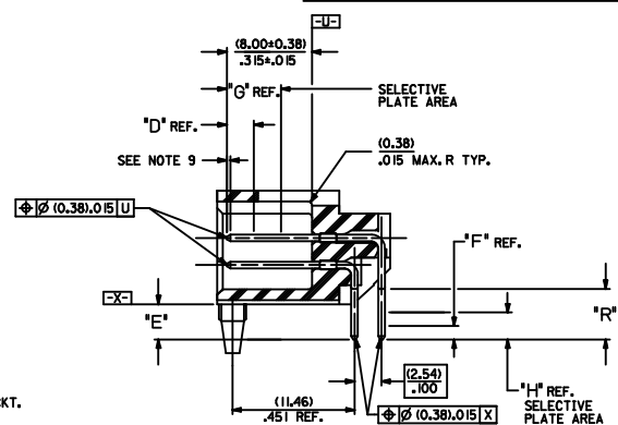
SECTION Z-Z
