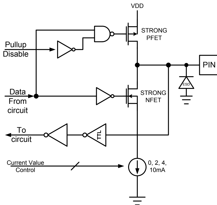
Figure 39: LED Circuit
