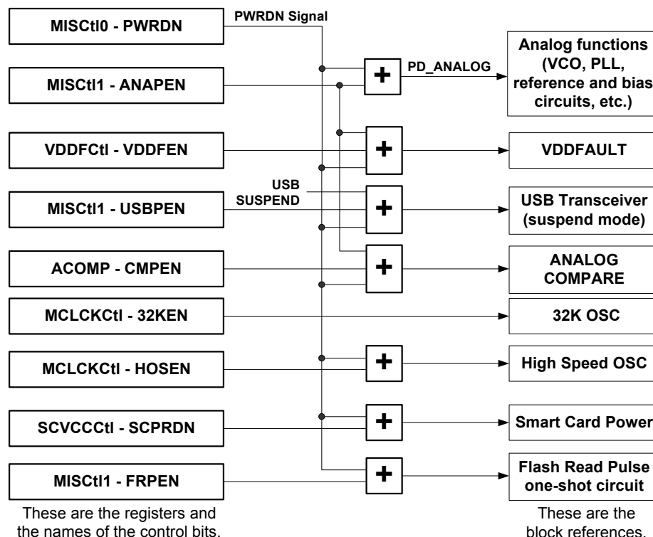
Figure 6: Power-Down Control
