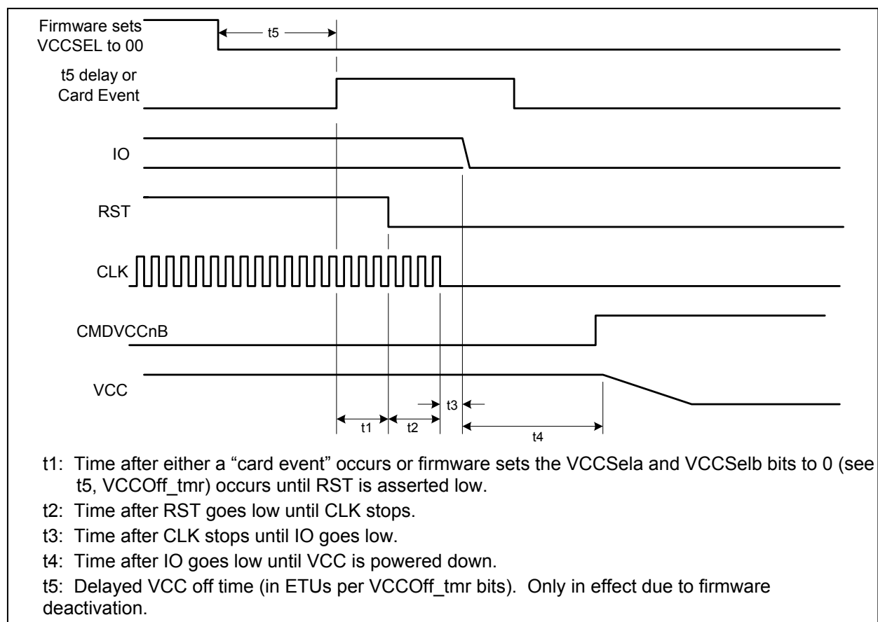
Figure 19: Deactivation Sequence
