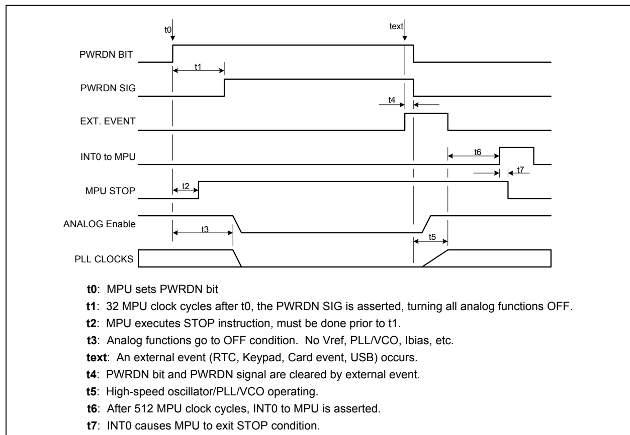
Figure 8: Power-Down Sequencing
