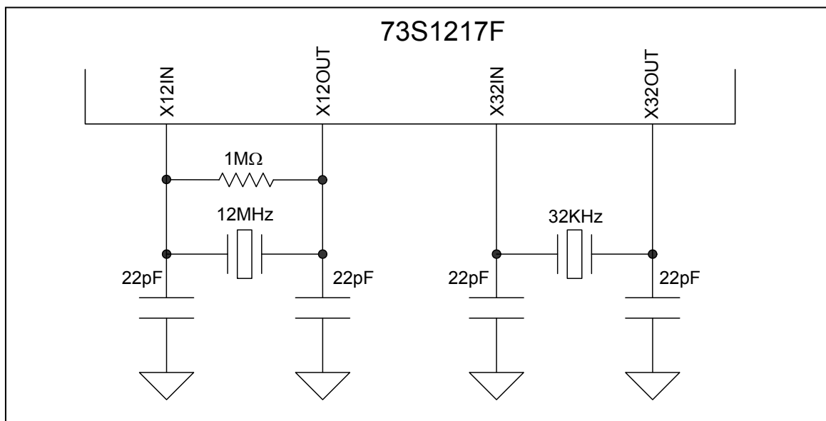
Figure 4: Oscillator Circuit
