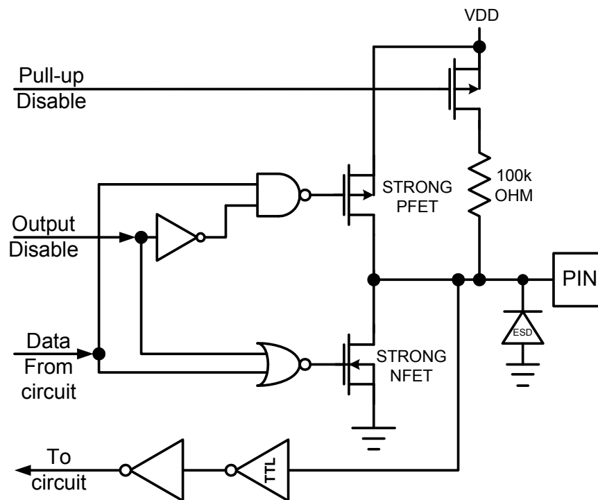
Figure 34: Keypad Row Circuit
