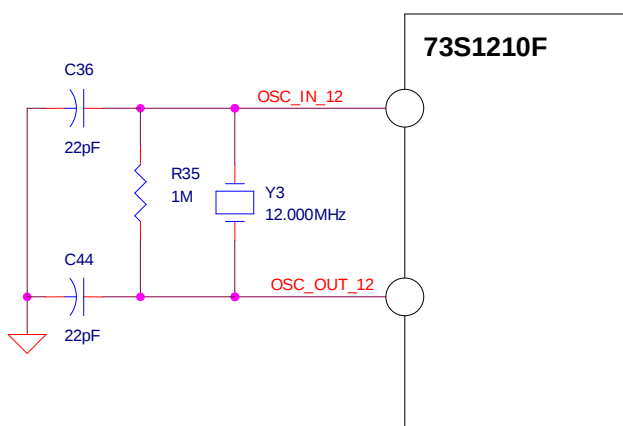
Figure 14: Oscillator Circuit
