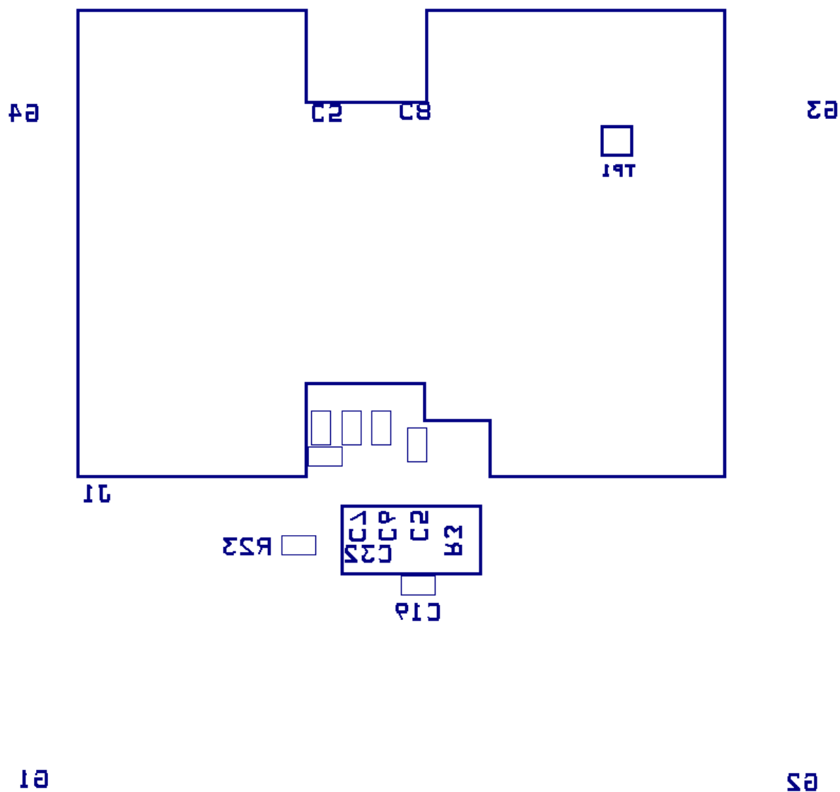
Figure 8: 73S1210F Evaluation Board Lite Bottom View (Silkscreen)
