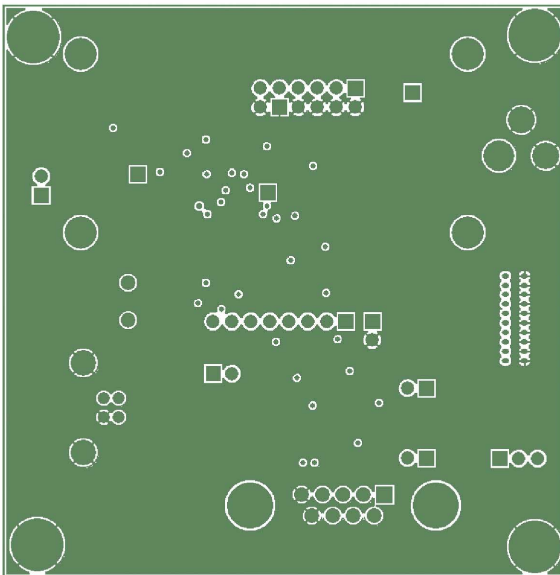
Figure 10: 73S1210F Evaluation Board Lite Middle Layer 1 – Ground Plane
