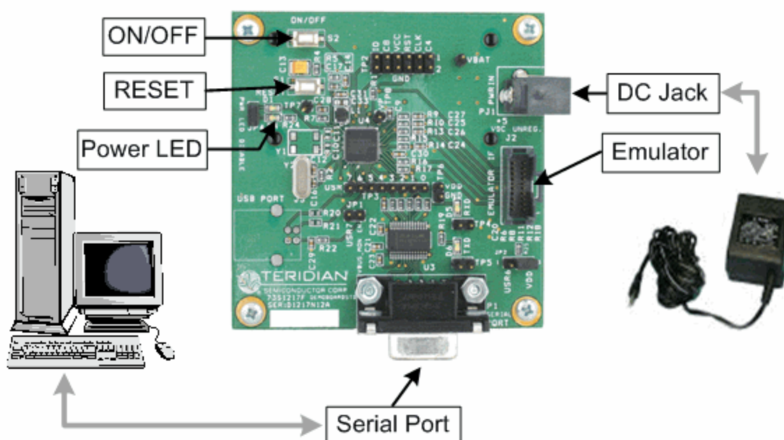
Figure 1: 73S1210F Evaluation Board-Lite Configuration
