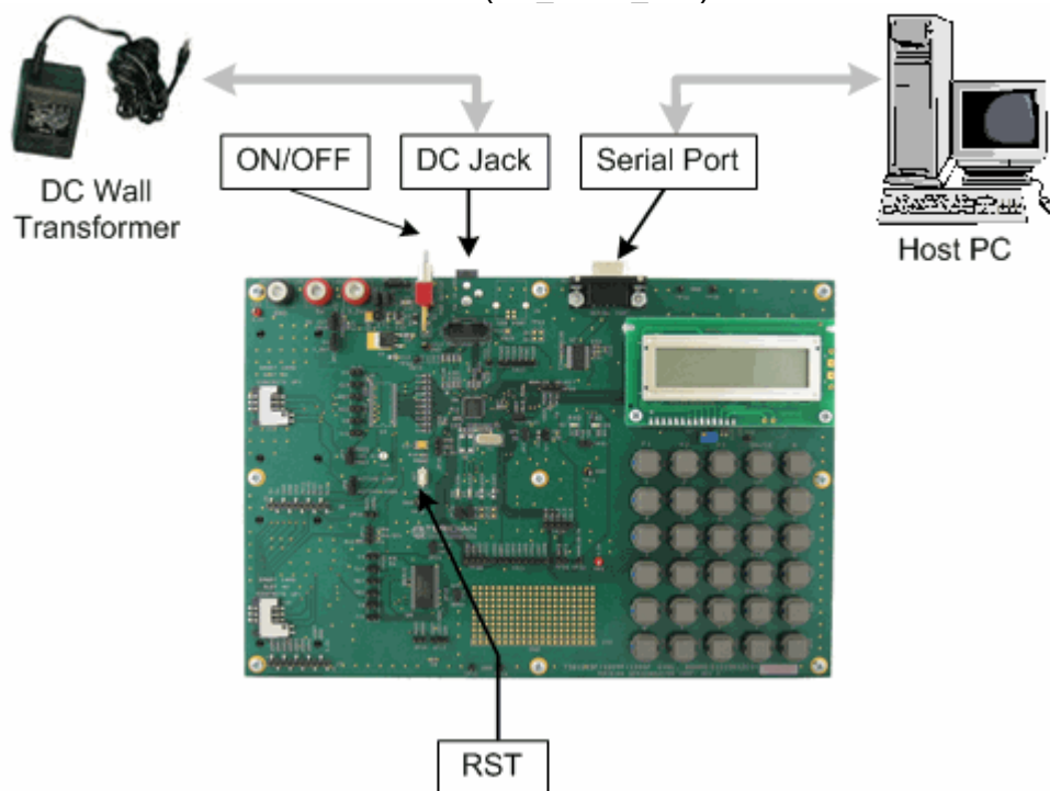
Figure 1: 73S1210F Evaluation Board Configuration
