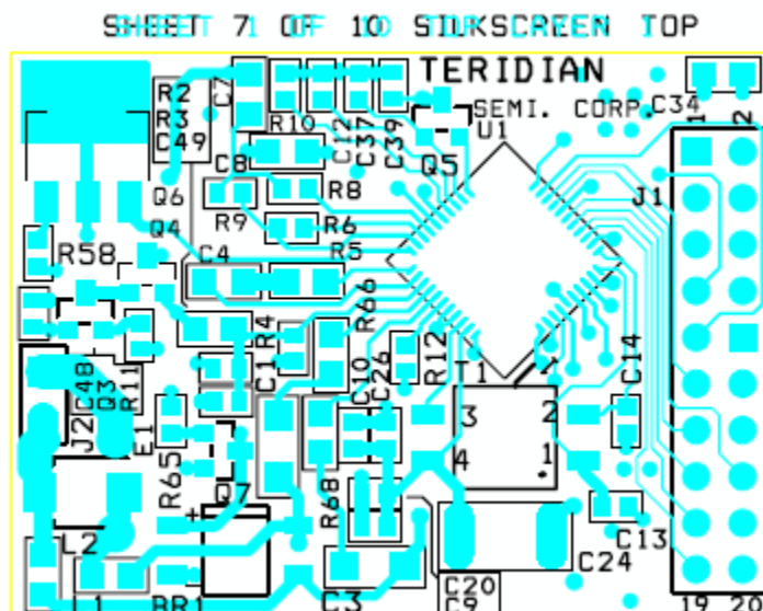
Figure 3: 73M1866B Keychain Demo Board Top Layer
