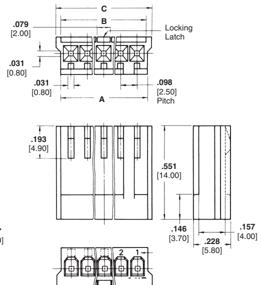
3-5 Position Housing
