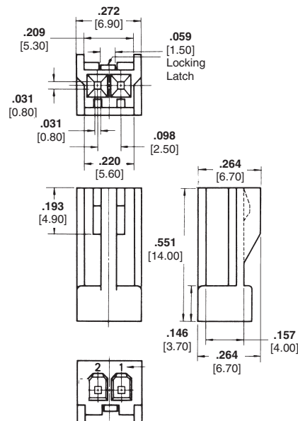
2 Position Housing
