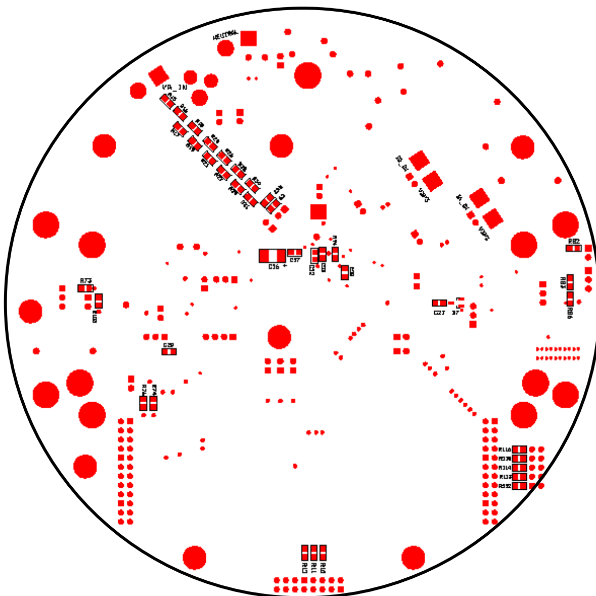
Figure 4-11: 71M6511 4-Layer Demo Board: Bottom View
