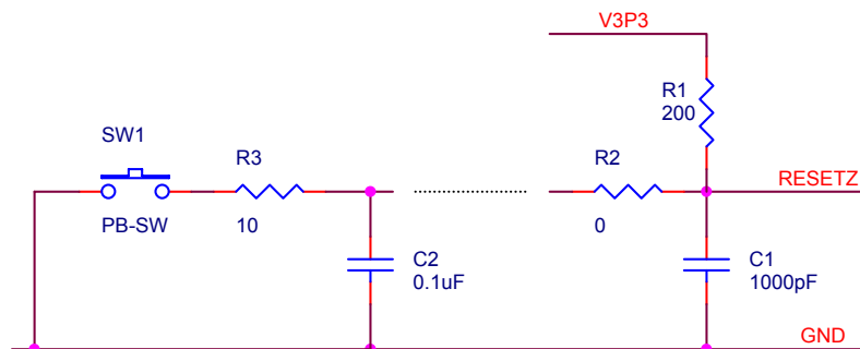
Figure 2-8: External Components for RESETZ
