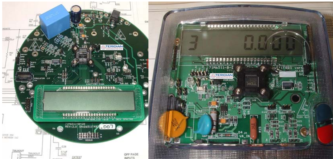
Figure 1-1: Demo Board Versions. 4-layer (left), 2-layer (right)
