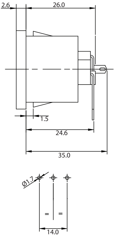
PCB FIXING DETAILS
