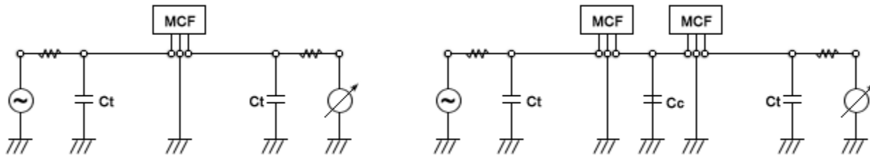
Figure 3) Test Circuits
