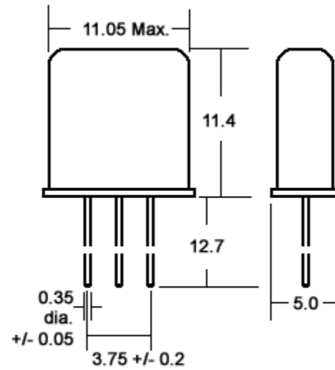
Figure 2) HC-49T
