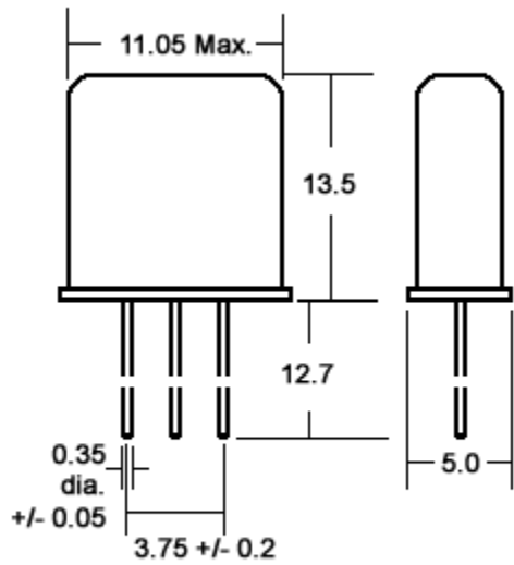
Figure 1) HC-49U
