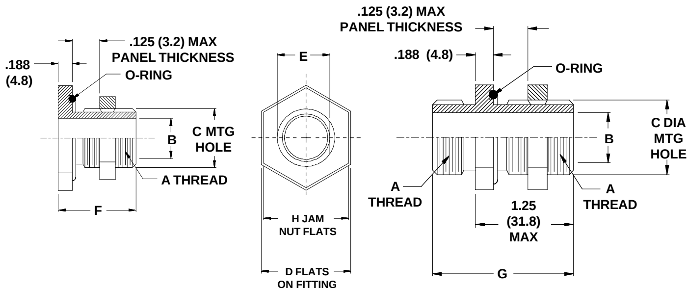
Bulkhead Adapters 710-100/101/372
