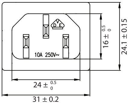
PANEL CUTOUT
