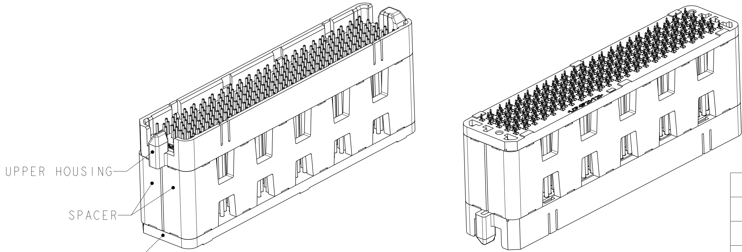
ISOMETRIC VIEWS TYPICAL CONFIGURATION FOR 14mm THRU 42mm 28mm SHOWN SCALE 2:1
