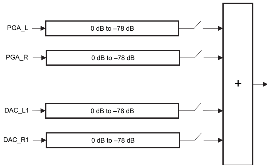
Figure 16. Detail of Volume Control and Mixing Function Shown in Figure 12 and Figure 24
