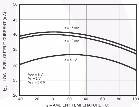
Figure 6. Low Level Output vs. Ambient Temperature
