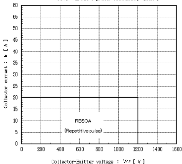
Reversed biased safe operating area V_{CE}=15V, T_J \leq 125^{\circ}C [Main Terminal] (min.)
