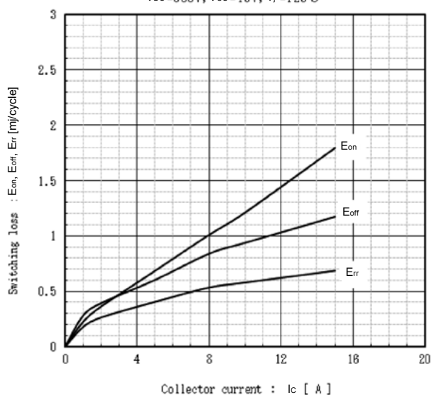
Switching Loss vs. Collector Current (typ.) V_{DC}=600V, V_{CE}=15V, T_J=125^{\circ}C
