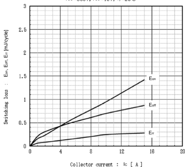
Switching Loss vs. Collector Current (typ.) V_{DC}=600V, V_{CE}=15V, T_J=25^{\circ}C
