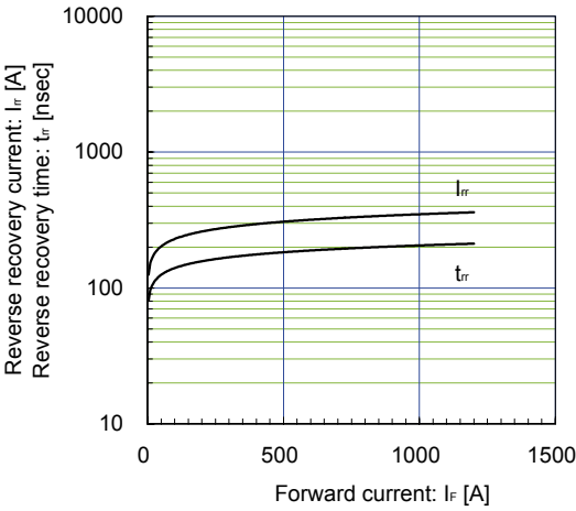
Reverse Recovery Characteristics (typ.) V CE =600V, V GE =±15V, R G =0.62Ω, T J =25°C
