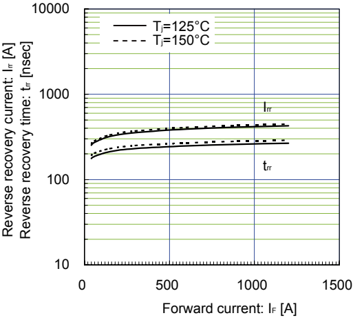
Reverse Recovery Characteristics (typ.) V CE =600V, V GE =±15V, R G =0.62Ω, T J =125°C, 150°C
