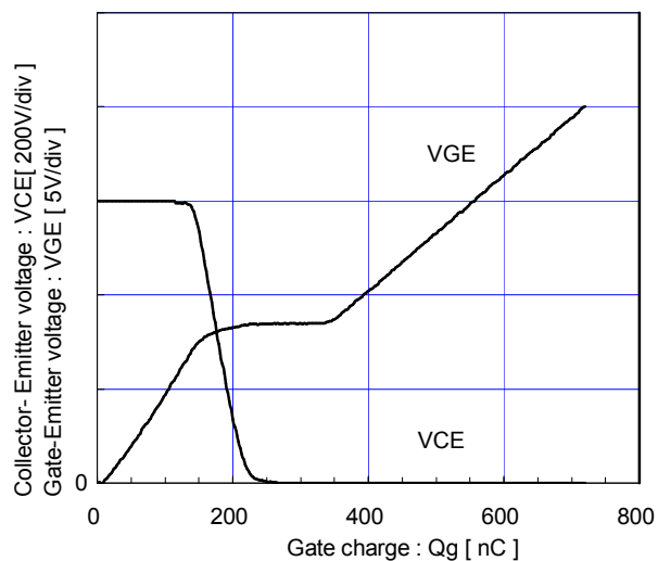
Dynamic Gate charge (typ.) Vcc=600V, Ic=150A, Tj=25°C
