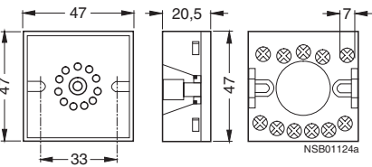
7PX9921 socket accessory with rear connection
