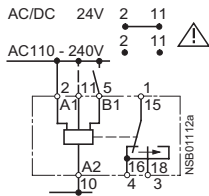
Pulse-forming with auxiliary voltage (B)
