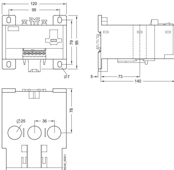
3UF7 113 current/voltage measuring module (straight-through transformer)
