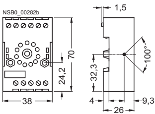
LZX:MT78750 socket accessory, for 7PV33
