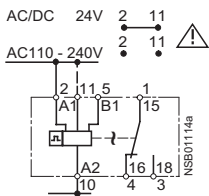
Flashing, starting with pulse (Di)
