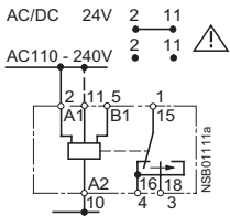
Passing make contact (H)
