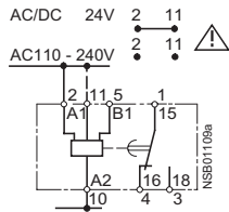
ON-delay (A)
